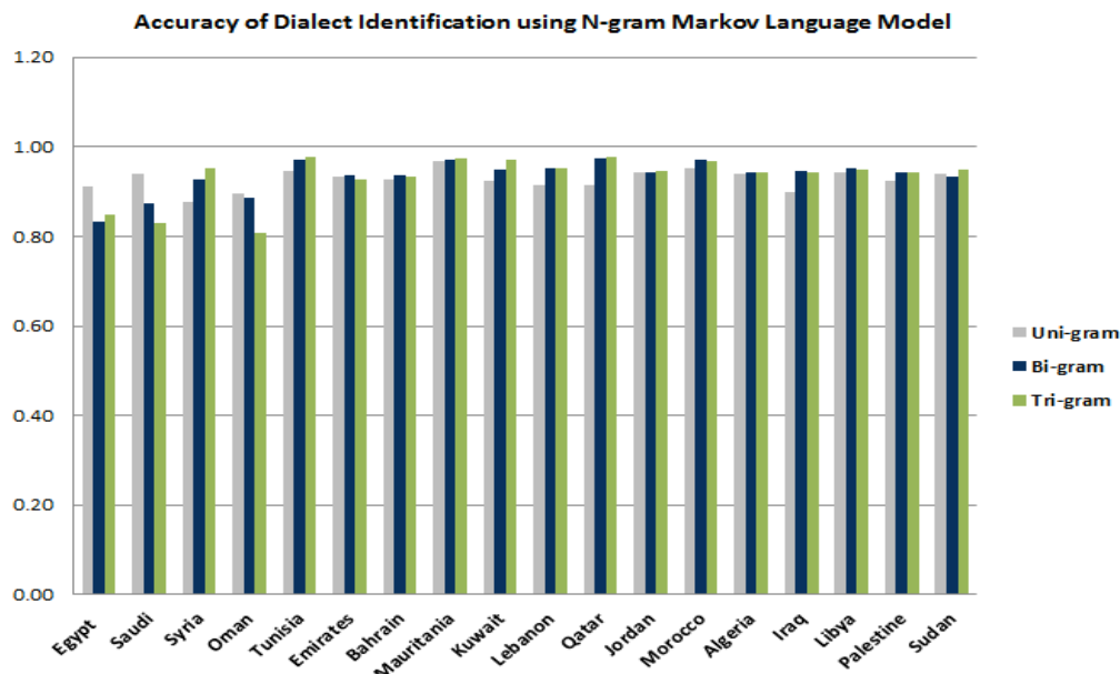
Figure 3. Accuracies on the character-based n-gram Markov language models for 18 countries
