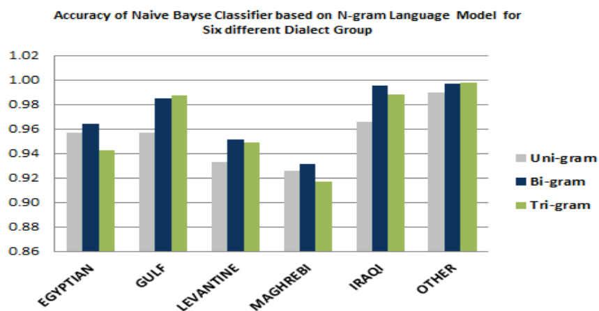
Figure 6. Accuracies on the character-based n-gram Naïve Bayes classifiers for the six divisions/groups
