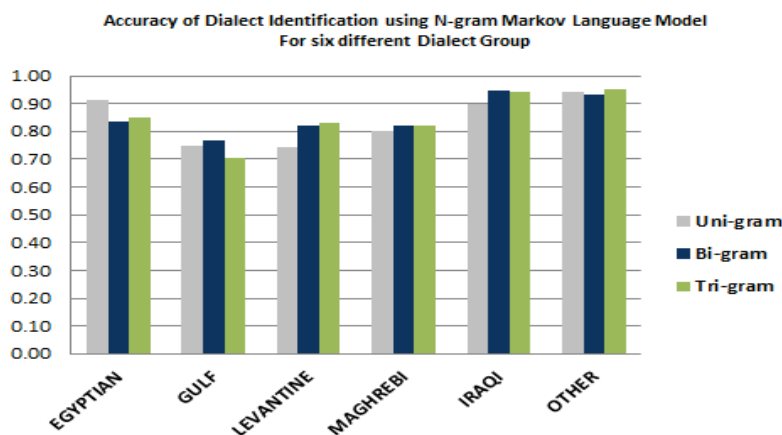
Figure 4. Accuracies on the character-based n-gram Markov language models for the six divisions/groups
