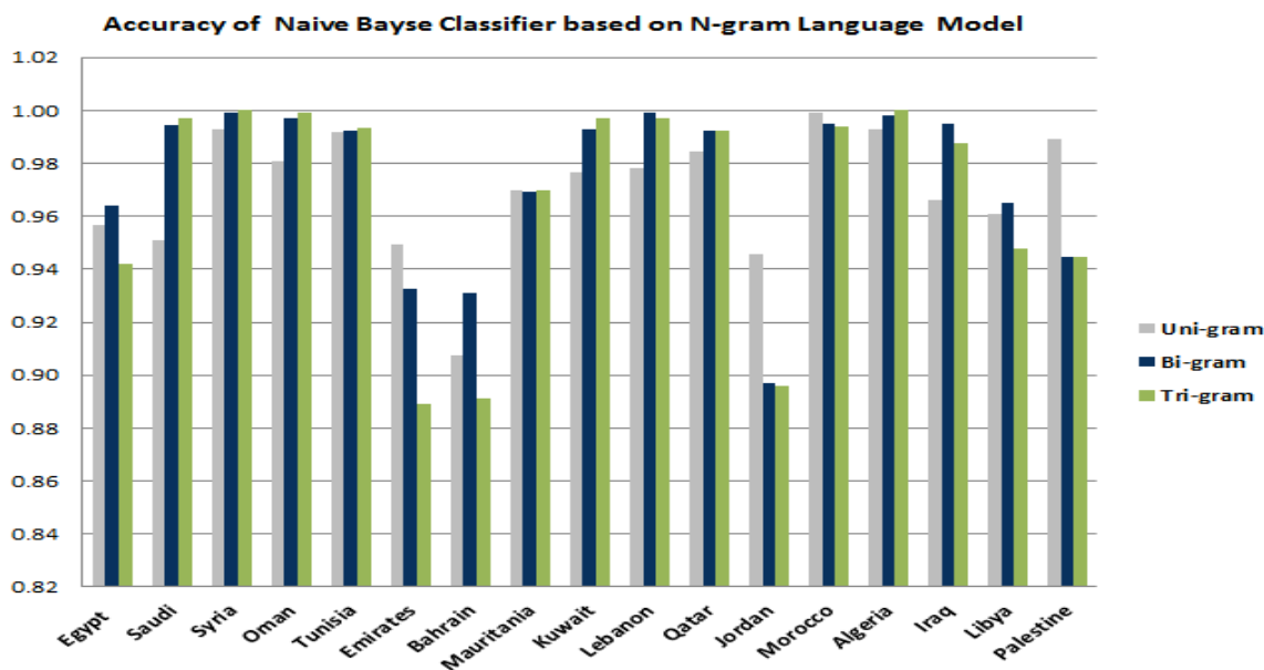
Figure 5. Accuracies on the character-based n-gram Naïve Bayes classifiers for 18 countries
