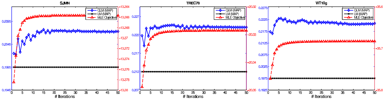
Figure 5: Plots of MAP (QLM-UNI and LM) and MLE objective against the number of updates of the density matrix for SJMN, TREC7-8 and WT10g (left, center and right).
