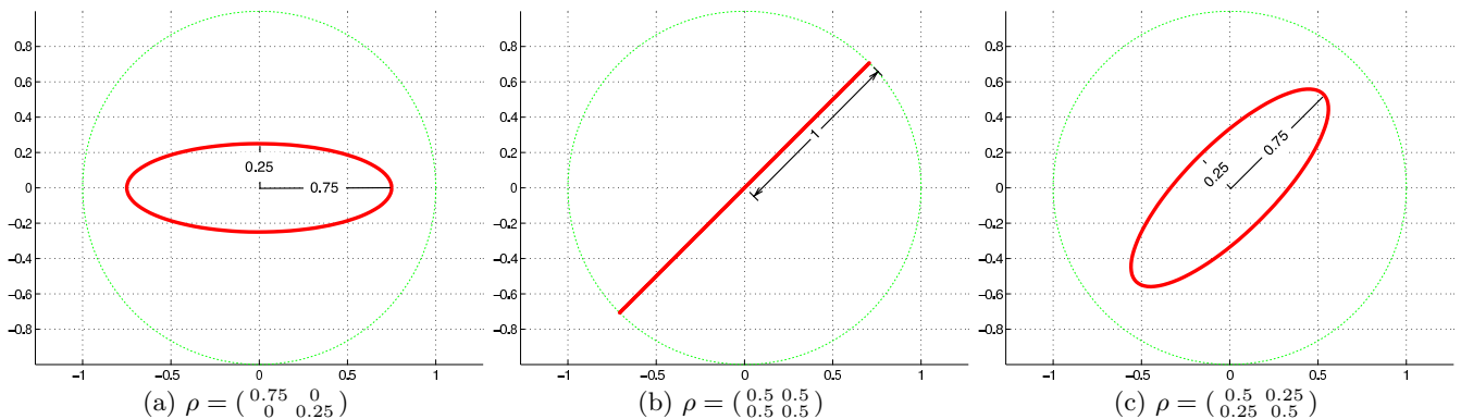
Figure 1: The ellipses depict the set of points \{\rho|u\rangle\langle u| : |u\rangle \in \mathbb{R}^2\} . The eigenvalues of \rho define how much each ellipse is stretched along the corresponding eigenvectors. To the left, \rho corresponds to a classical probability distribution. To the center, \rho is a pure state, thus the ellipse degenerates along the eigenvector corresponding to its unit eigenvalue. To the right, a general density matrix for which we vary both the eigenvalues and the eigensystem.
