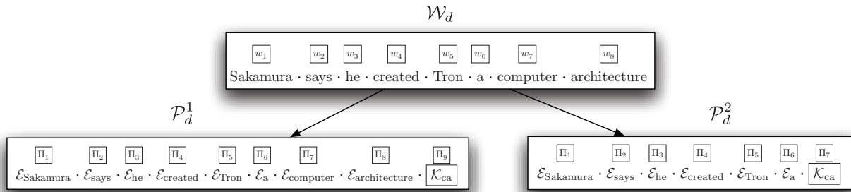
Figure 3: Two possible quantum sequences \mathcal{P}_d^i of an excerpt \mathcal{W}_d from a TREC collection. The observation of computer architecture is associated to a superposition projector \mathcal{K}_{ca} = |\kappa_{ca}\rangle\langle\kappa_{ca}| while \mathcal{E}_w = |e_w\rangle\langle e_w| are classical projectors. For \mathcal{P}_d^2 we observed only the compound while in \mathcal{P}_d^1 we also added its subsets.
