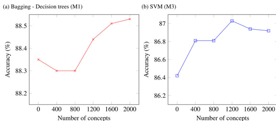
FIGURE 1 Accuracy of decision trees with bagging (M1) and support vector machine (SVM) (M3) using concepts
