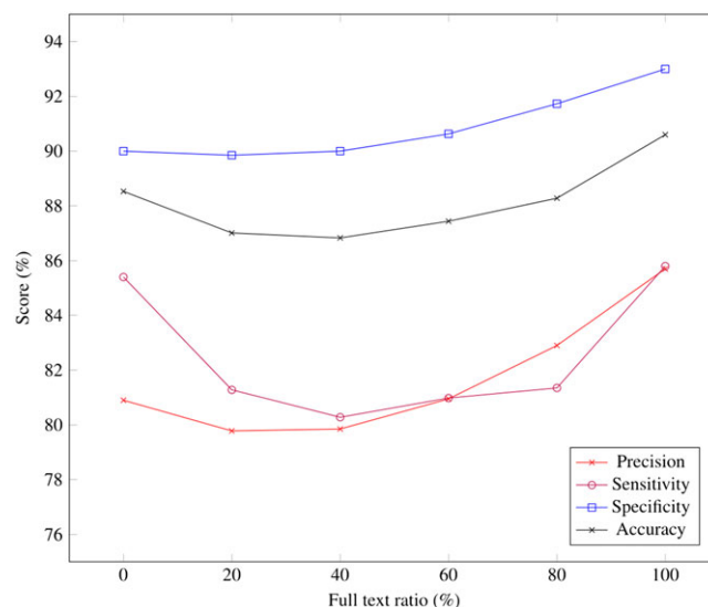
FIGURE 3 Performances of decision trees with bagging (M1) mixing abstracts and full texts
