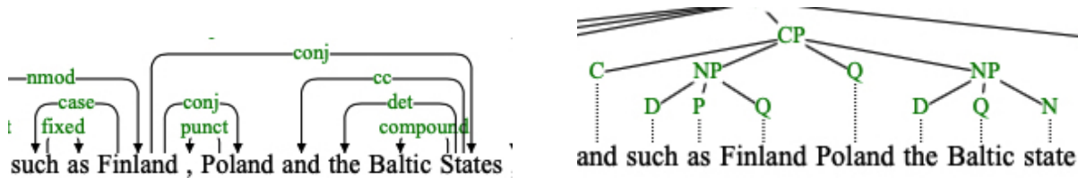
Figure 4: The graph at the left, a subgraph of the UD w02013093 in en_pud-ud-test.conllu , illustrates the UD encoding of coordinated nouns Finland , Poland and the Baltic States ; the right part shows the expected dependency tree by JSREALB .
