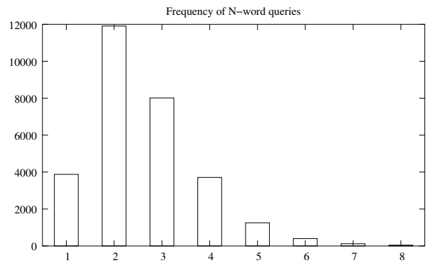
Figure 4: Distribution of queries as a function of their size
