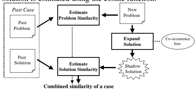
Figure 1 - Case similarity using co-occurrence lists
