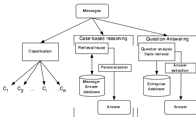
Fig. 6. Modules of the Mercure Project
