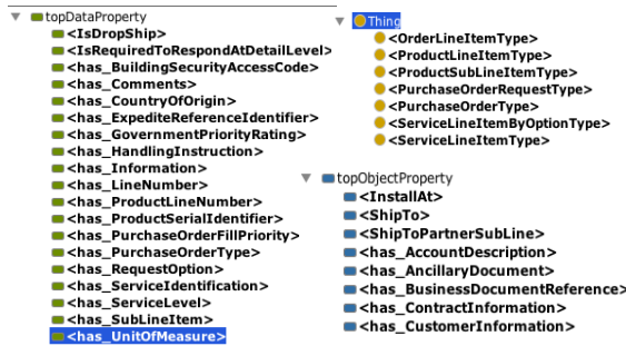
Figure 2: Screen prints tabs from Protégé describing the PIP3A4 Ontology generated by XSD2OWL Mapping (Classes, Data Properties and Object Properties).
