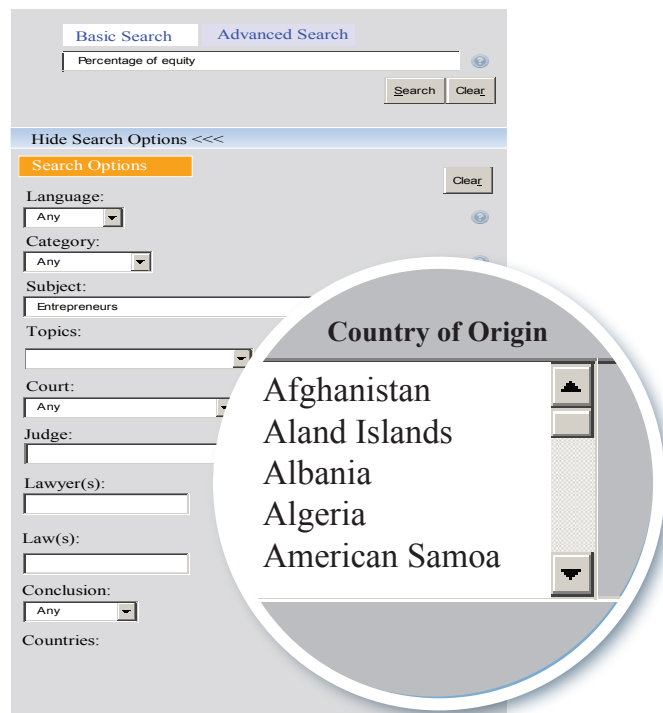
Fig. 3. With SearchExpress , it is possible to have access to relevant decisions for a research in progress by specifying the criteria. For example a lawyer can carry out a research on a precise case such as an entrepreneur who comes from a certain country with the particular conditions to see how such situations have been treated historically in order to calculate the chance of success in court.
