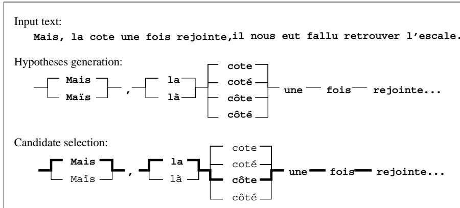
Figure 1: Automatic accent insertion method
